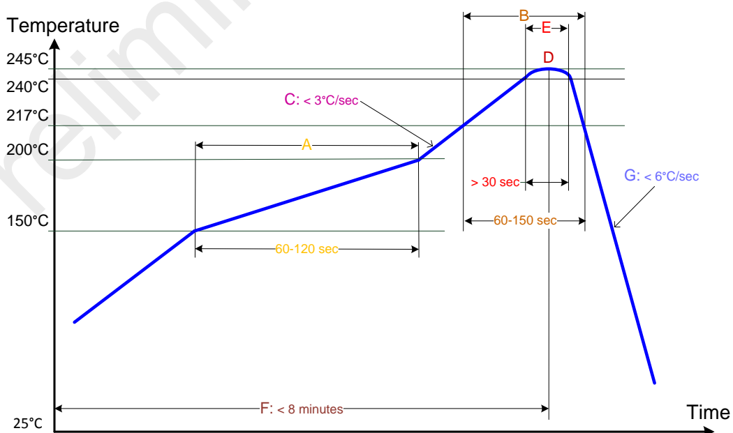
Figure 6-4 Soldering Profile
